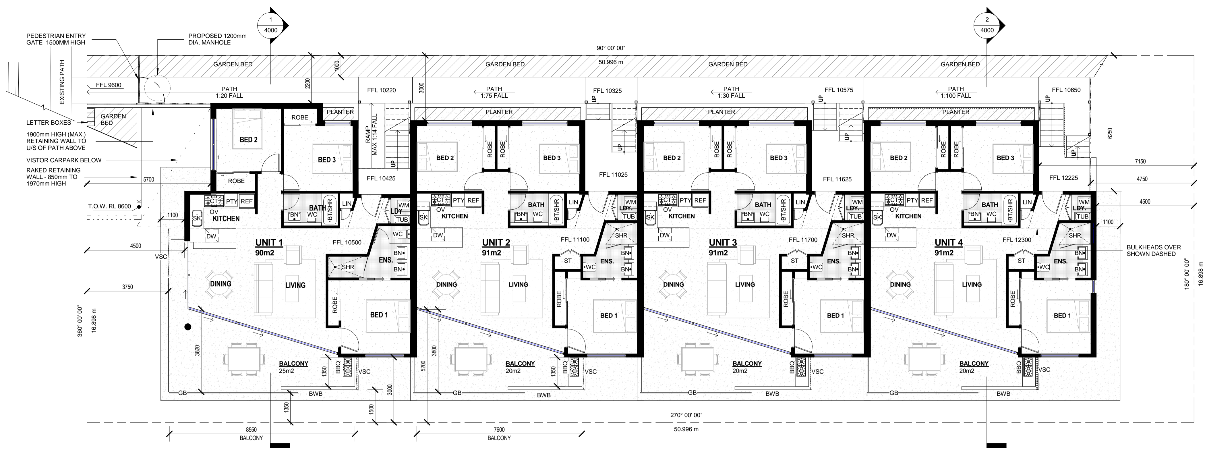
1 FIRST FLOOR 1:100
