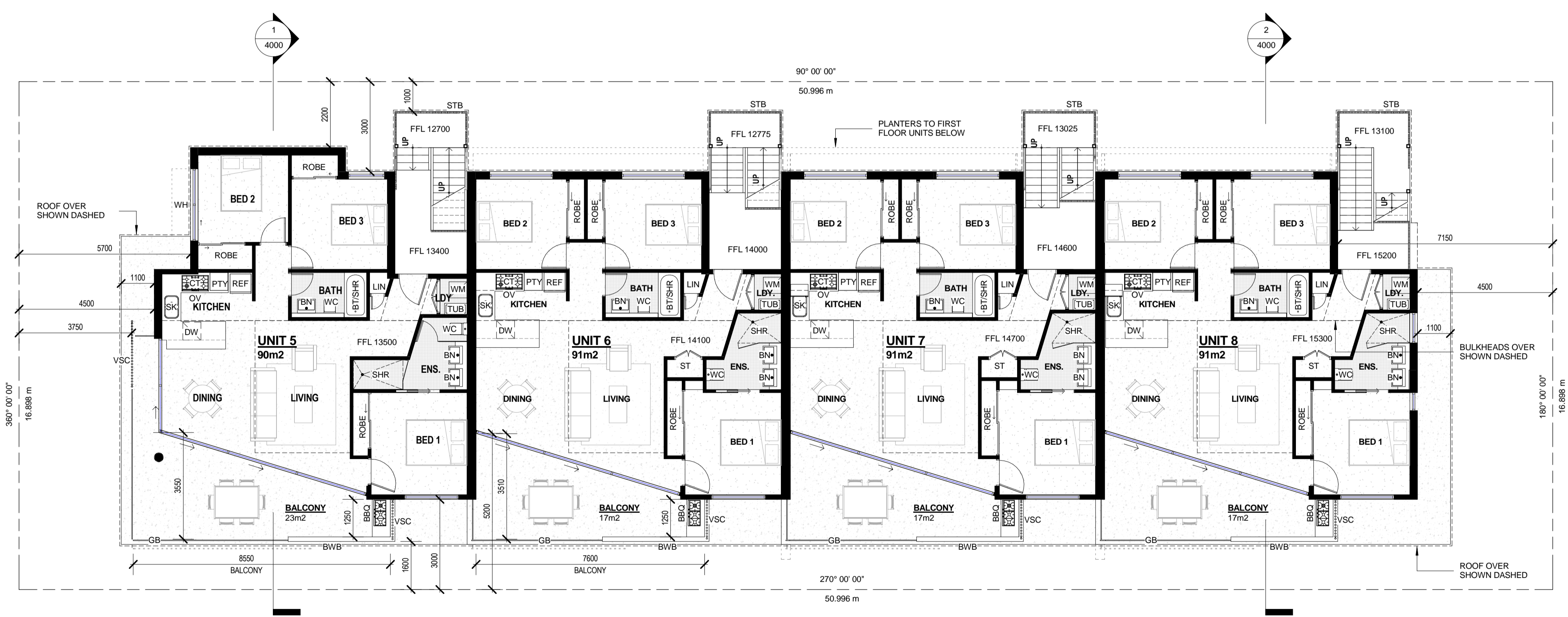
2 SECOND FLOOR 1:100
